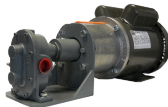
Model 6LOI with Single Phase TEFC Motor
